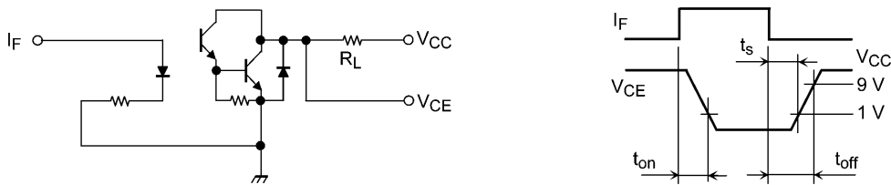
Fig. 10.1 Switching Time Test Circuit
